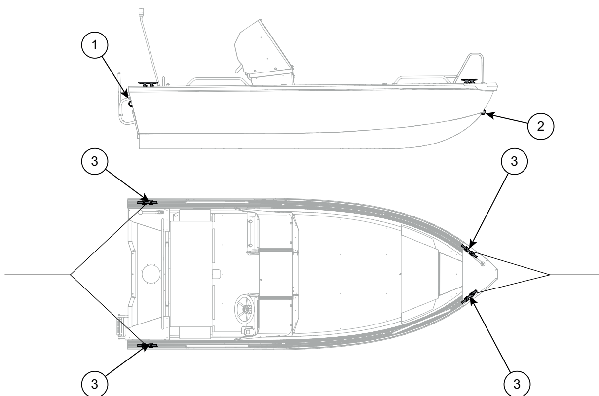
Figure 5.4 Buster S/S1/S2/Sc mooring and towing point
