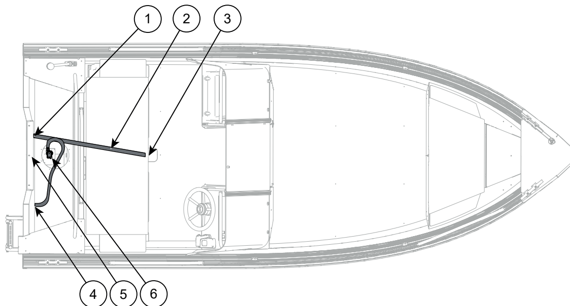
Figure 9.2 Buster S1/S2/Sc locations of draining equipment
