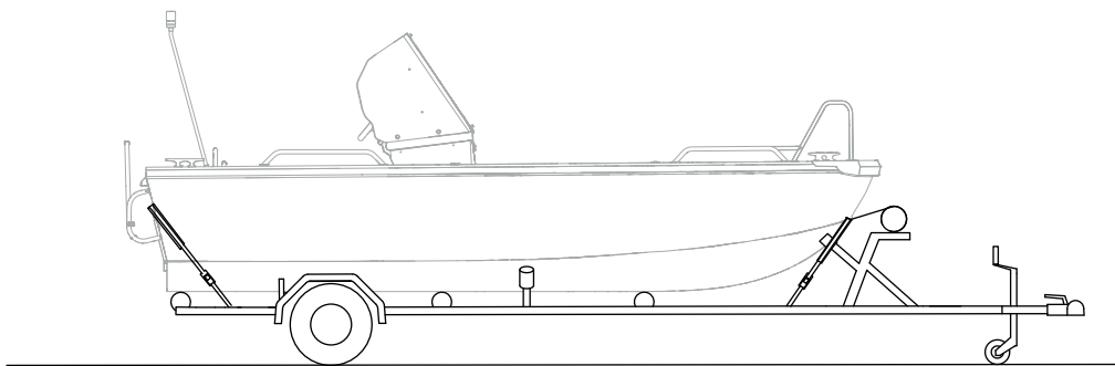
Figure 12.1 Buster S/S1/S2/Sc placement on the trailer
