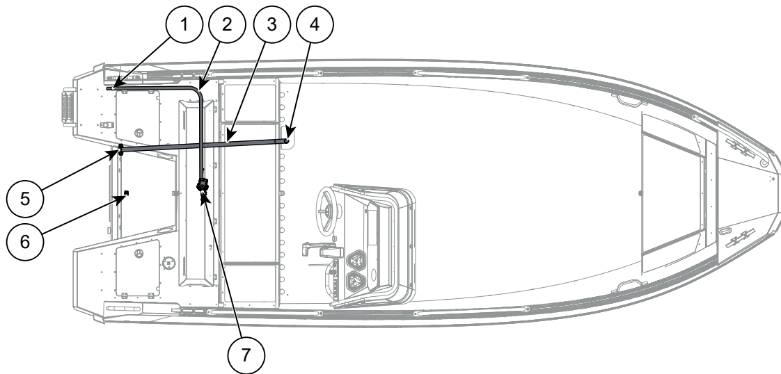
Figure 9.1 Buster L1/L2/Lcc locations of draining equipment
