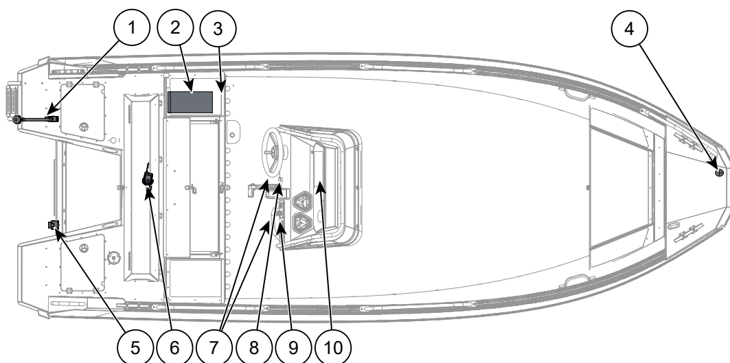
Figure 8.6 Buster Lcc electrical equipment
