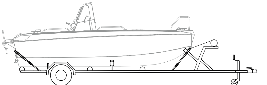
Figure 12.1 Buster L1/L2/Lcc trailer transportation
