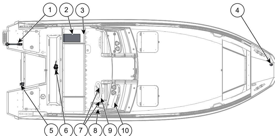
Figure 8.5 Buster L2 electrical equipment
