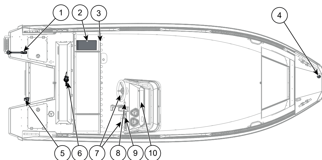
Figure 8.4 Buster L1 electrical equipment
