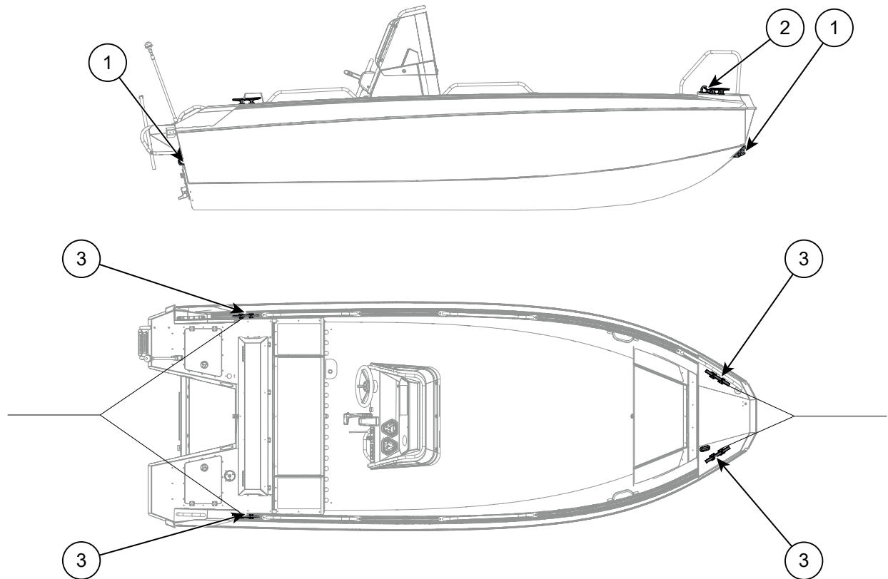
Figure 5.5 Buster L1/L2/Lcc mooring and towing points
