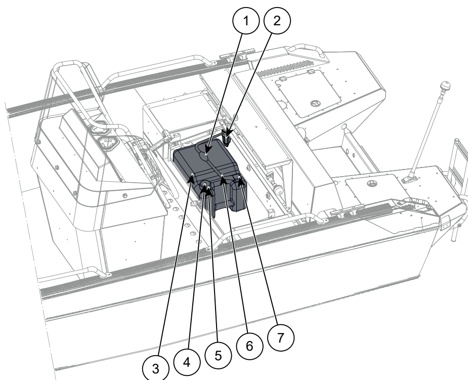
Figure 6.1 Buster L1/L2/Lcc fuel system with removable fuel tank
