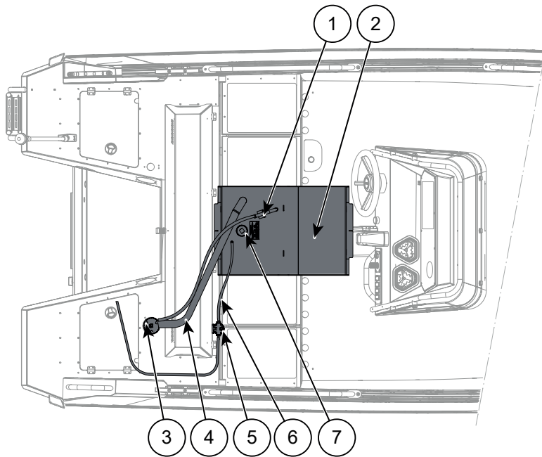
Figure 6.2 Buster L1/L2/Lcc fuel system with optional fixed fuel tank
