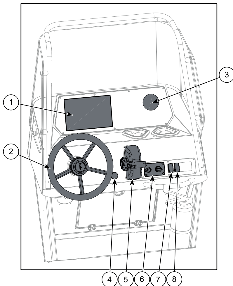
Figure 5.1 Buster L1/Lcc helm station controls
