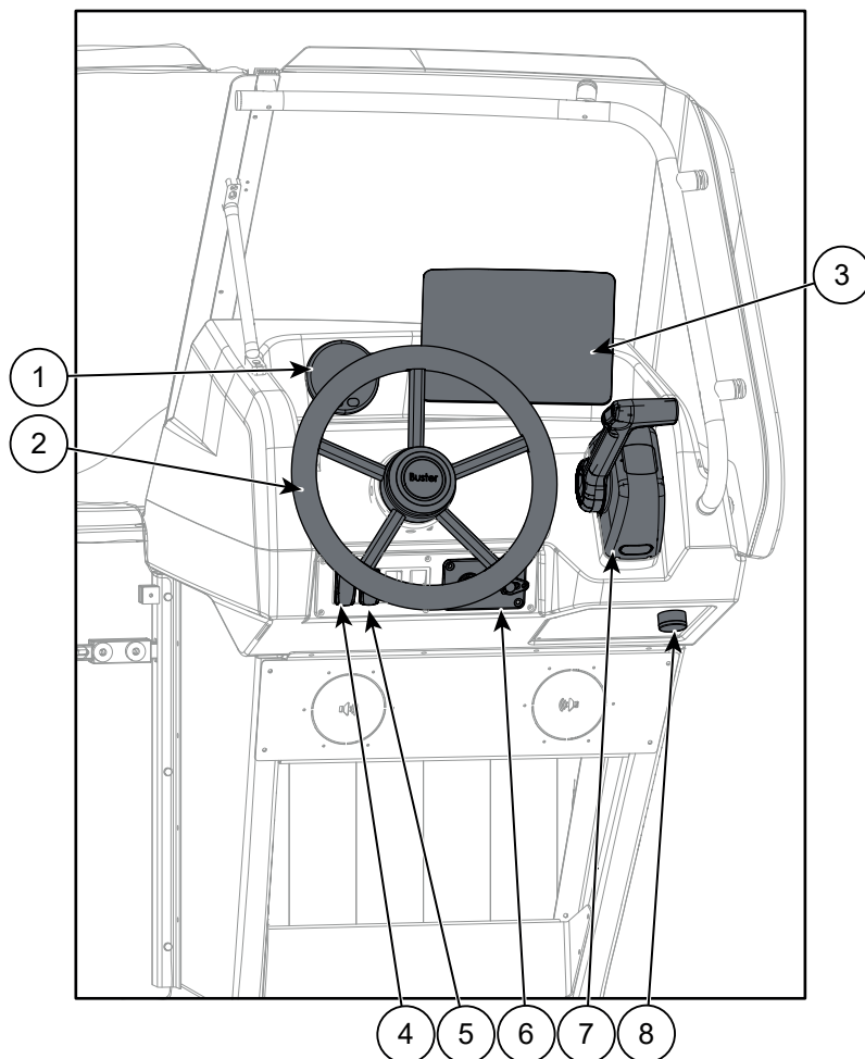
Figure 5.2 Buster L2 helm station controls
