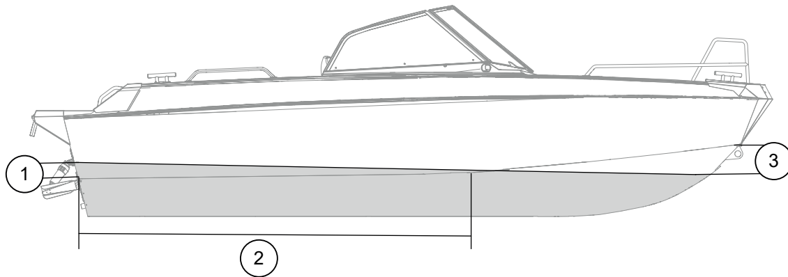
Figure 3.1 Buster XL/XLcc/XXL/XXLcc antifouling paint area
