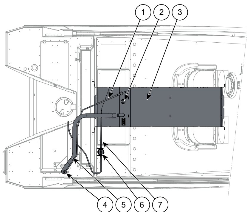
Figure 6.1 Buster XL/XLcc/XXL/XXLcc fuel system components
