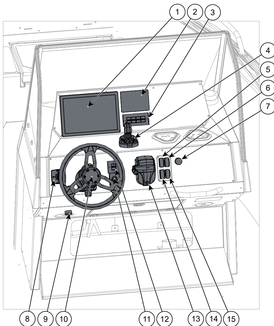
Figure 5.2 Buster XLcc/XXLcc helm station controls
