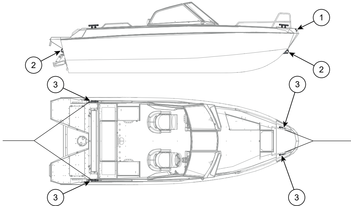
Figure 5.8 Buster XL/XLcc/XXL/XXLcc mooring and towing points
