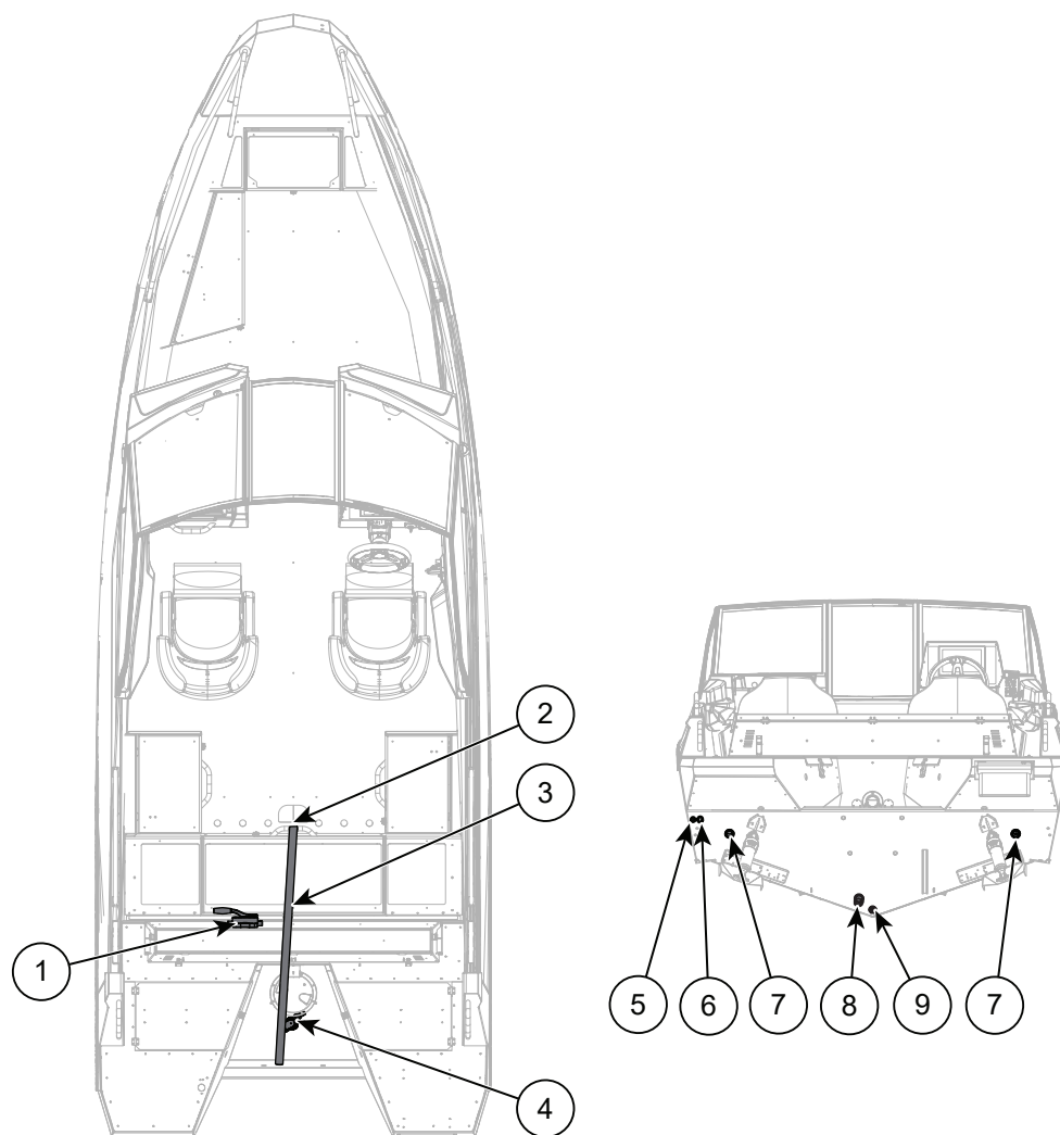
Figure 9.1 Buster XL/XLcc/XXL/XXLcc draining equipment
