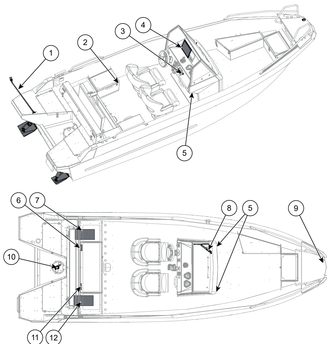
Figure 8.6 Buster XLcc/XXLcc electrical equipment
