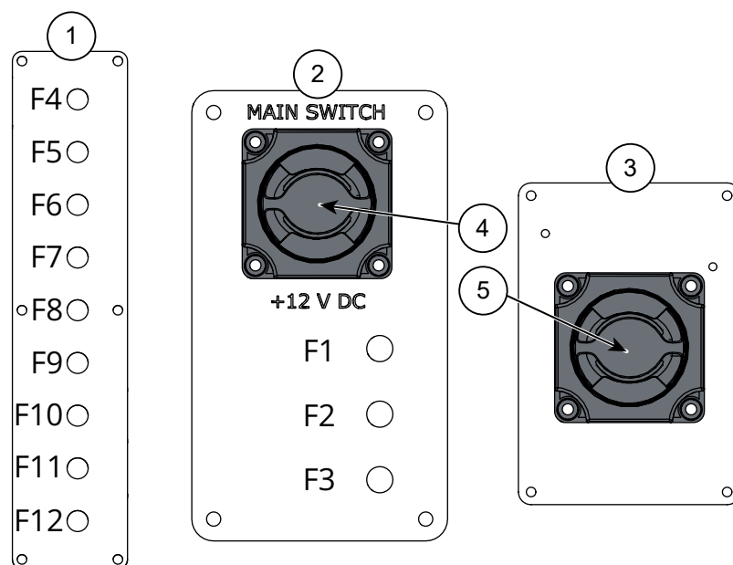
Figure 8.1 Buster XL/XLcc/XXL/XXLcc main switches and fuse panels
