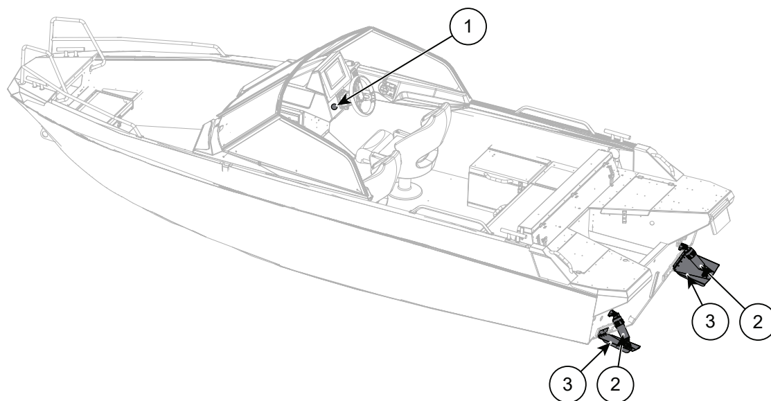
Figure 5.7 Buster XL/XLcc/XXL/XXLcc trim system components
