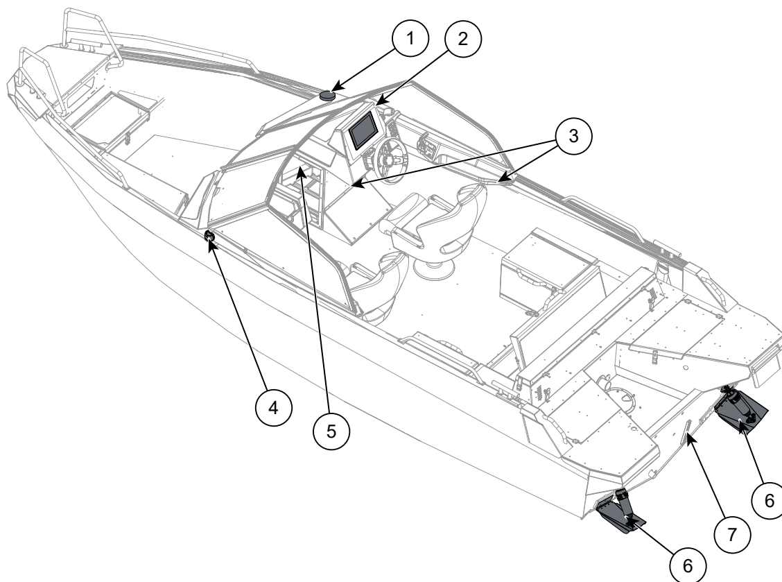
Figure 8.5 Buster XL/XXL electrical equipment
