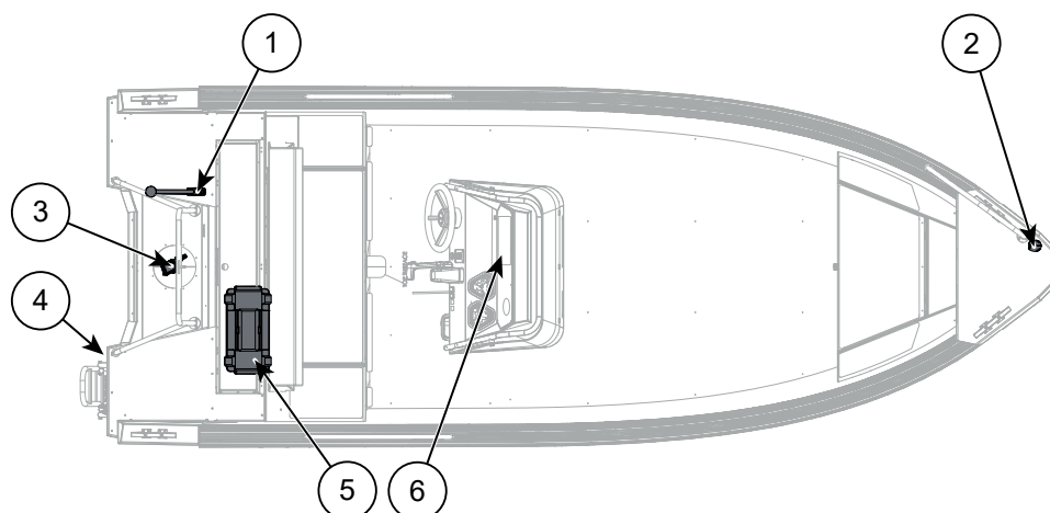
Figure 8.3 Buster Mcc electrical equipment
