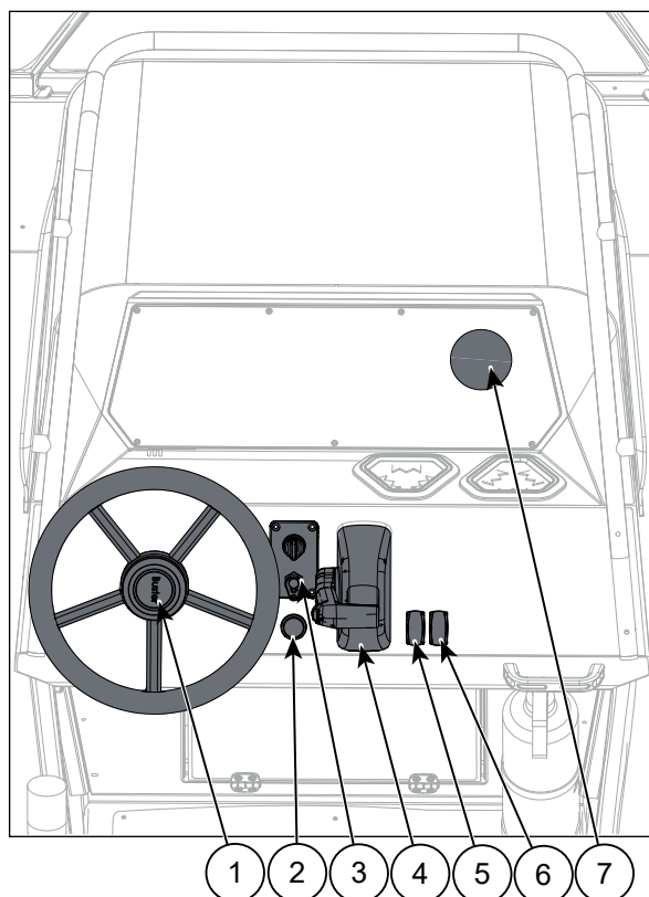
Figure 5.3 Buster Mcc helm station controls
