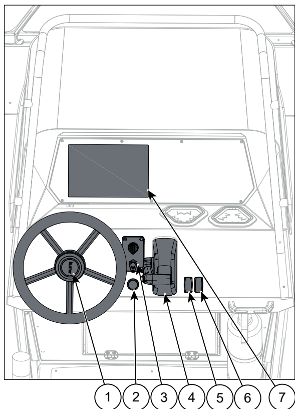
Figure 5.4 Buster Mcc helm station controls with Buster Q
