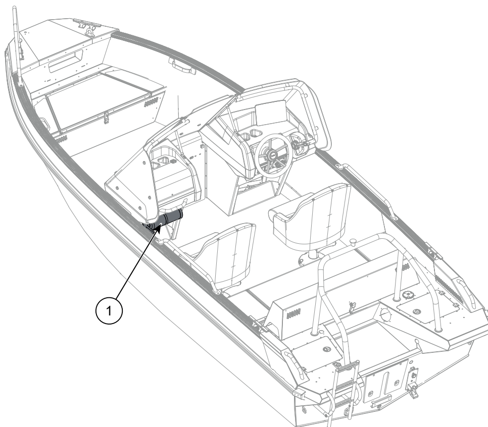
Figure 2.2 Buster Lx location of fire extinguisher
