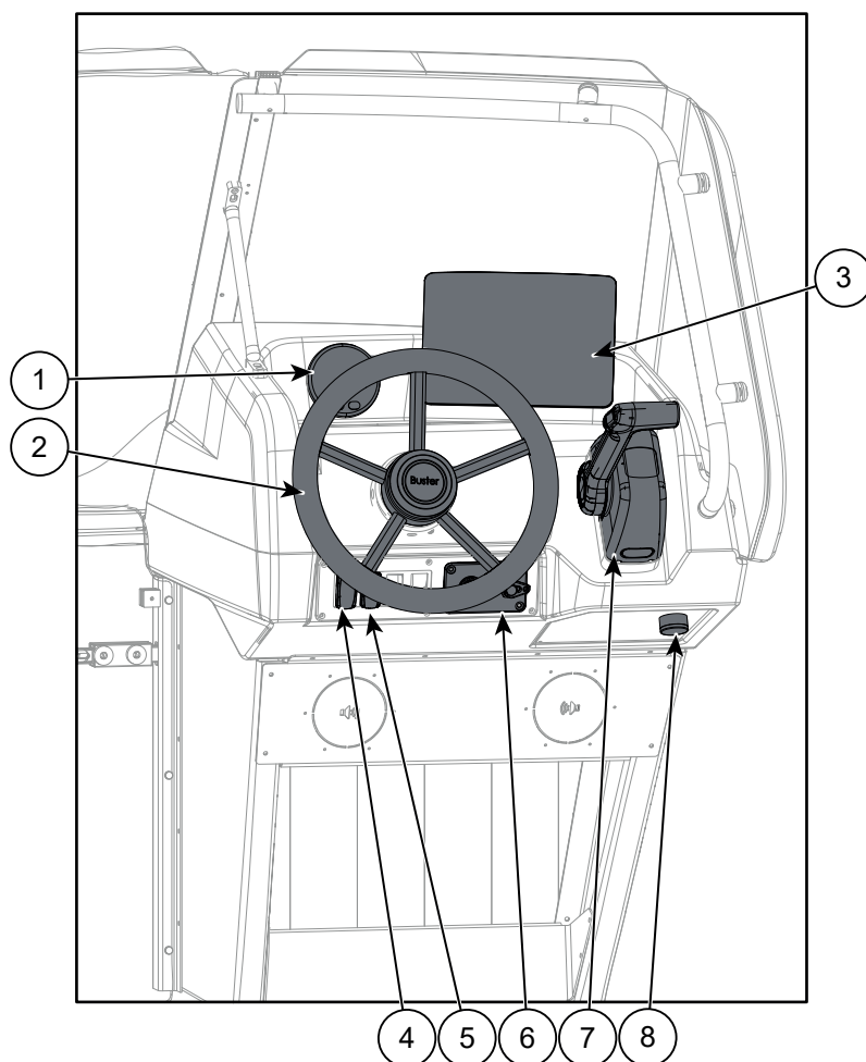
Figure 5.1 Buster Lx helm station controls
