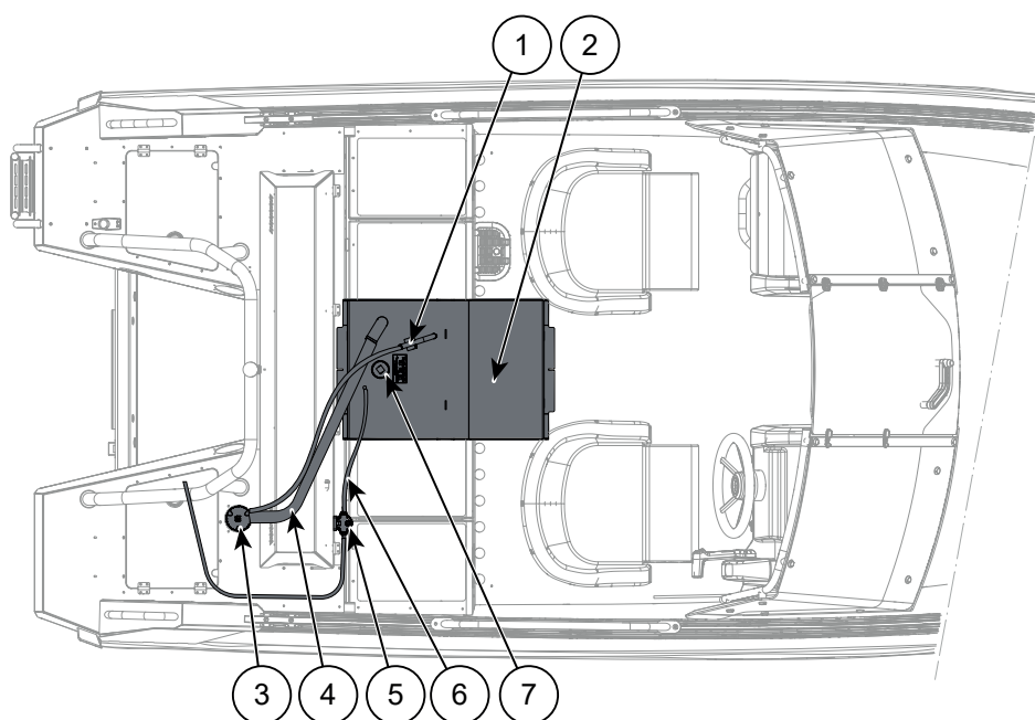
Figure 6.1 Buster Lx fuel system components
