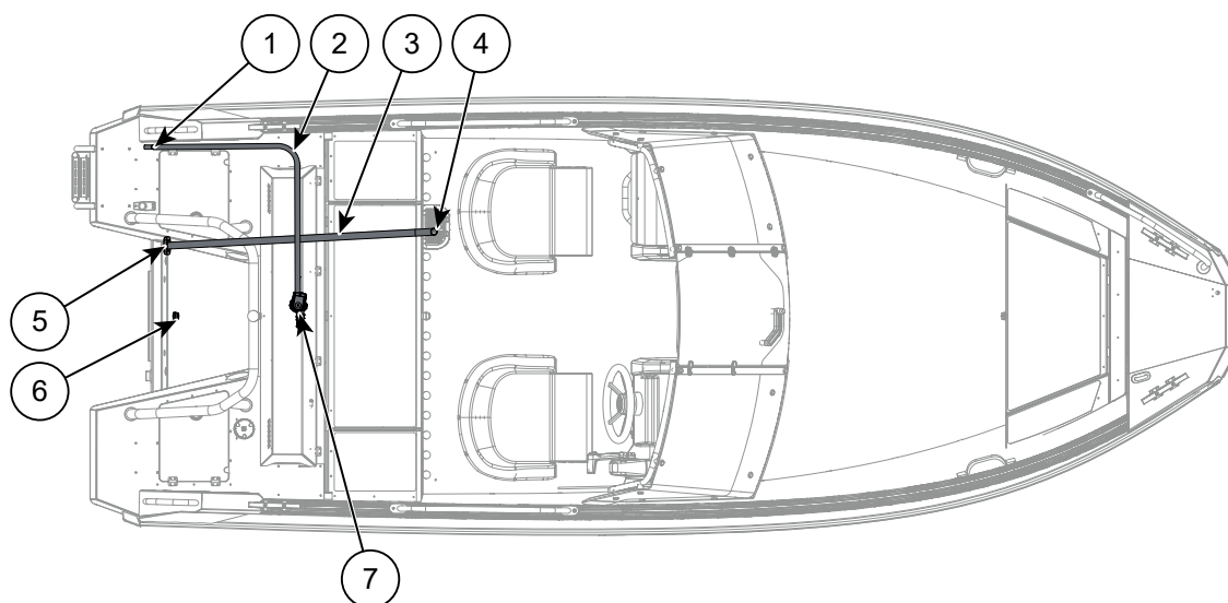
Figure 9.1 Buster Lx locations of draining equipment
