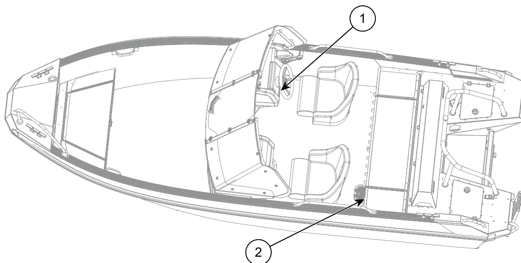
Figure 8.2 Buster Lx fuse panel locations
