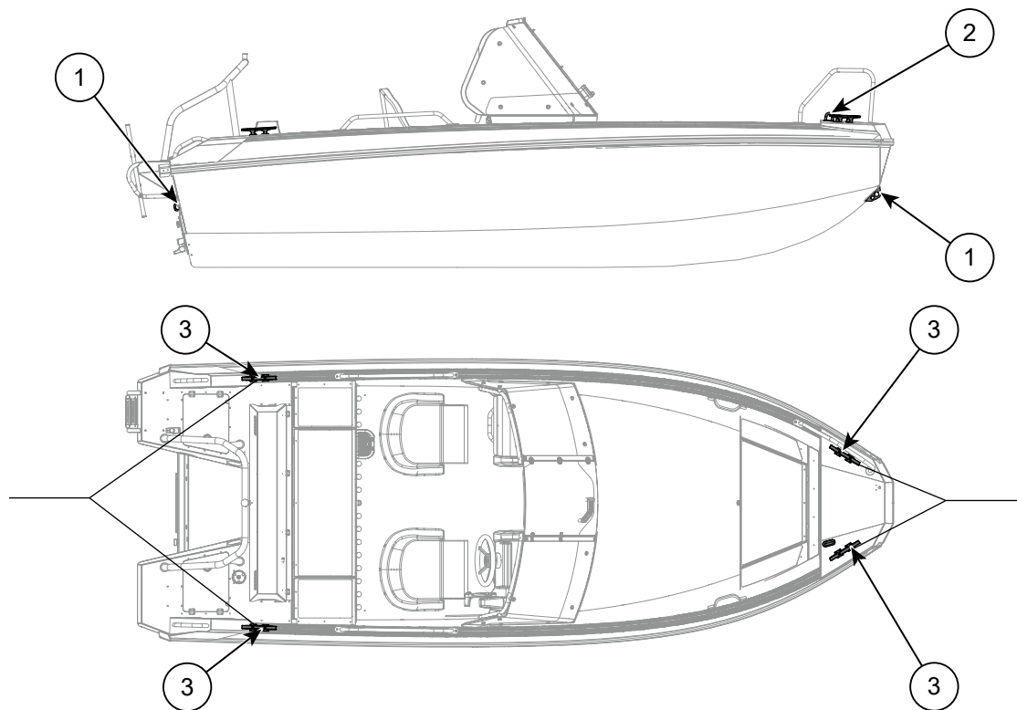
Figure 5.4 Buster Lx mooring and towing points
