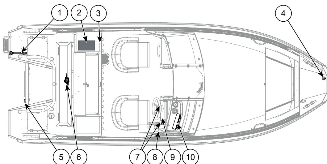
Figure 8.3 Buster Lx electrical equipment
