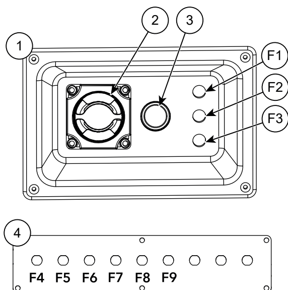
Figure 8.1 Buster Lx main switch and fuse panels
